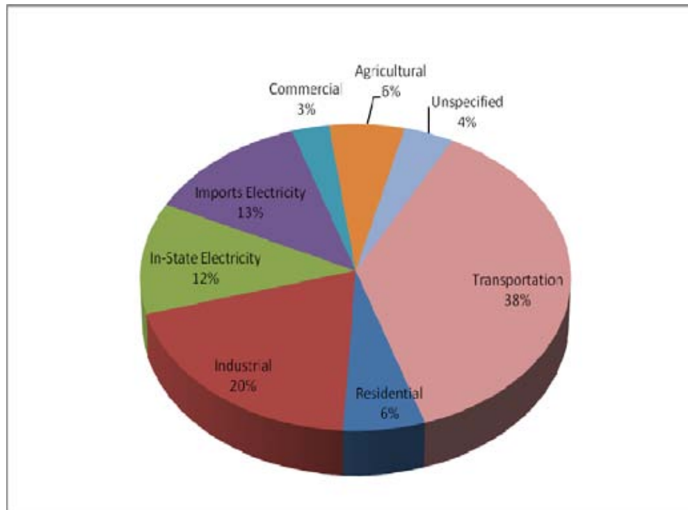
Figure 4-4. Sources of Greenhouse Gas Emissions – 2004
