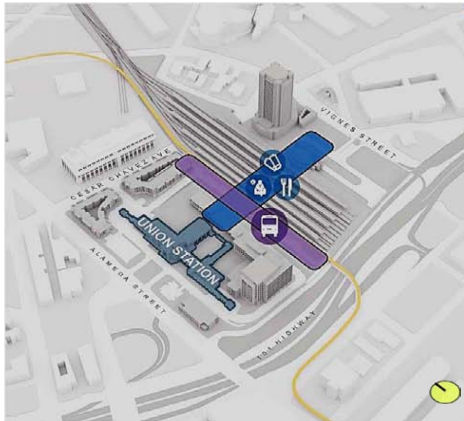
E/W Passenger Concourse + N/S Relocated Patsouras Bus Facility - RECOMMENDED
